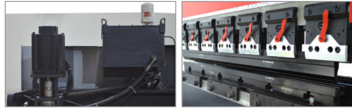
▲ Servo Hybrid Drive System
